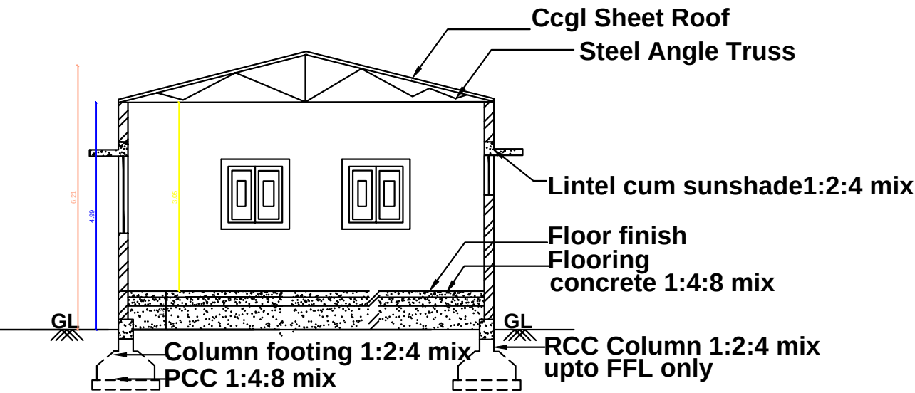
SECTION ELEVATION
