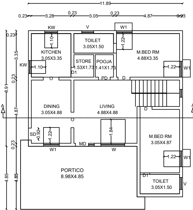
EXISTING GROUND FLOOR APPROVAL PLAN
