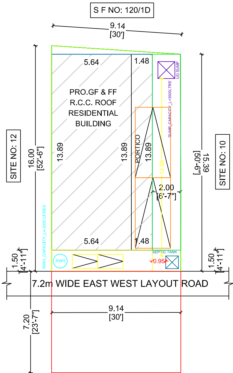
SITE PLAN
