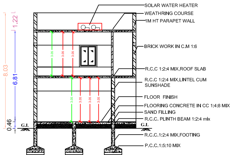
SECTION (B-B)
