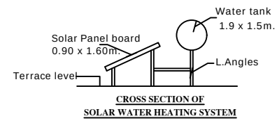
CROSS SECTION OF SOLAR WATER HEATING SYSTEM
