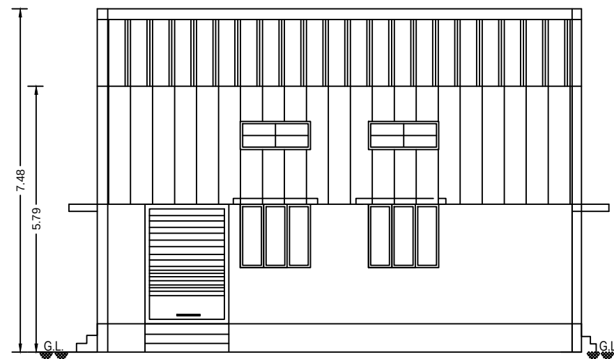
Elevation -North Side
