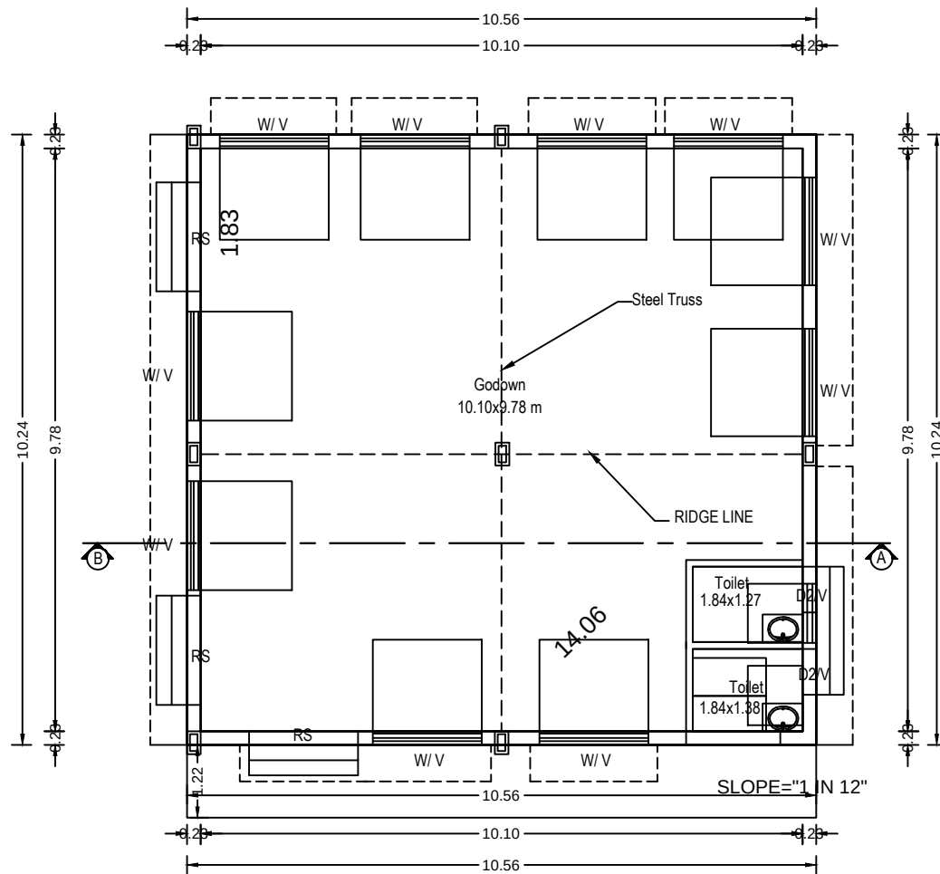
SCALE 1:100 GROUND FLOOR PLAN
