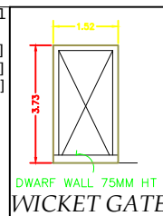
DWARF WALL 75MM HT WICKET GATE
