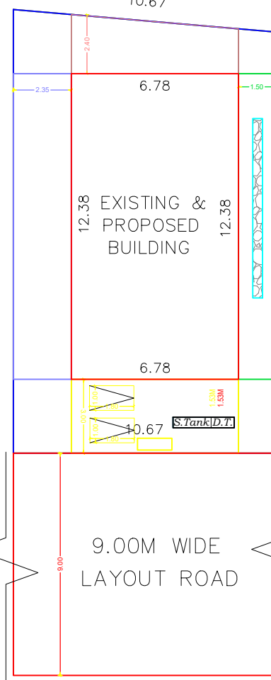
SITE PLAN
