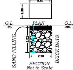
Trial - Pit (Not to Scale)
