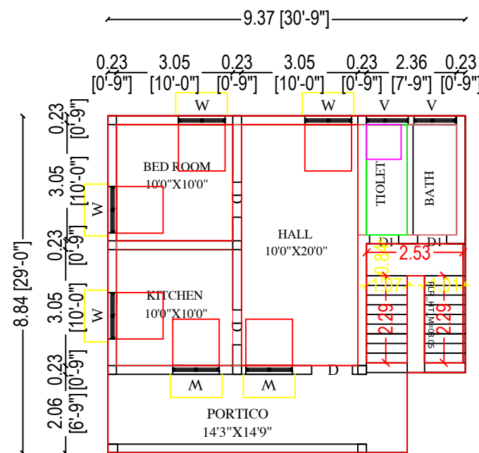
PROPOSED PLAN
