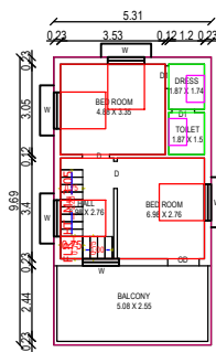
PROPOSED FIRST FLOOR BUILDING
