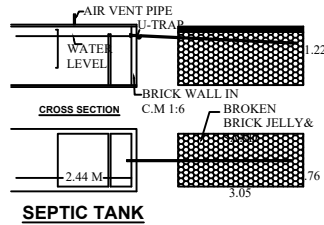
SEPTIC TANK
