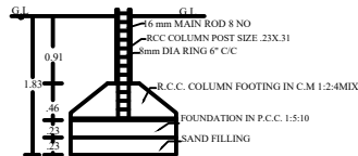
COLUMN POST DETAILS
