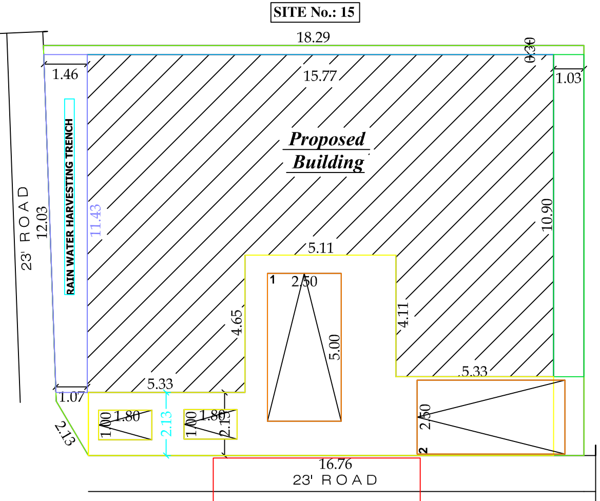
SITE PLAN
