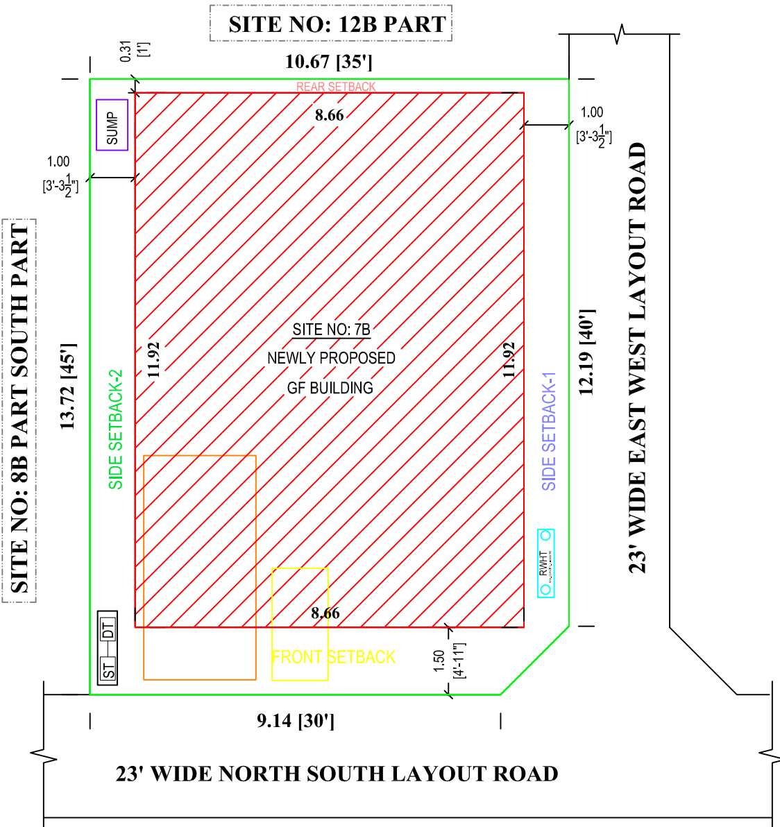
SITE PLAN
