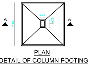
PLAN DETAIL OF COLUMN FOOTING
