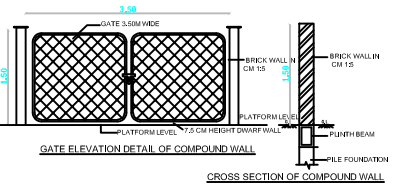
GATE ELEVATION DETAIL OF COMPOUND WALL
