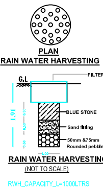
RAIN WATER HARVESTING (NOT TO SCALE)
