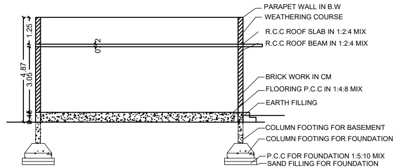
SECTION ON-AA
