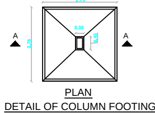
PLAN DETAIL OF COLUMN FOOTING
