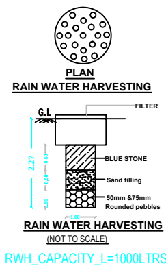
RAIN WATER HARVESTING (NOT TO SCALE) RWV_CAPACITY_L=1000LTRS
