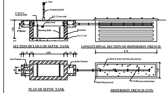
DETAILS OF SEPTIC TANK - 250 GALLONS & DISPERSION TRENCH
