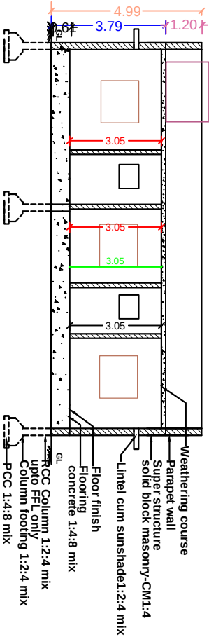
SECTION ELEVATION
