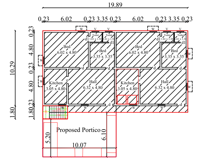
Plan for Existing & Proposed Ground Floor
