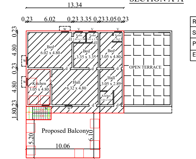
Plan for Existing First Floor & Proposed First Floor
