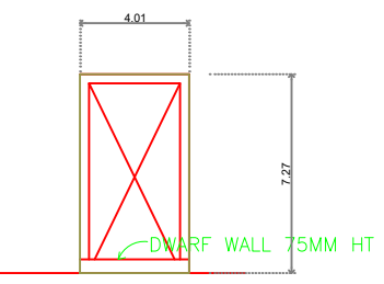
MAIN GATE ELEVATION
