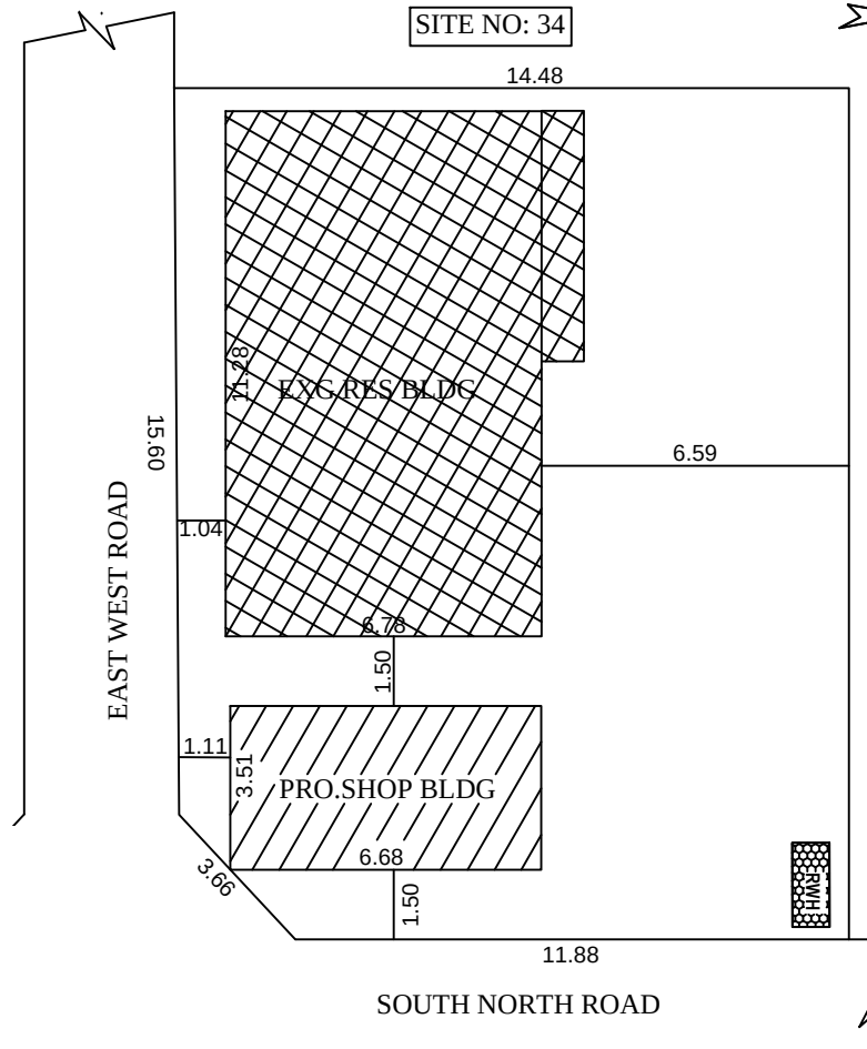
SITE PLAN
