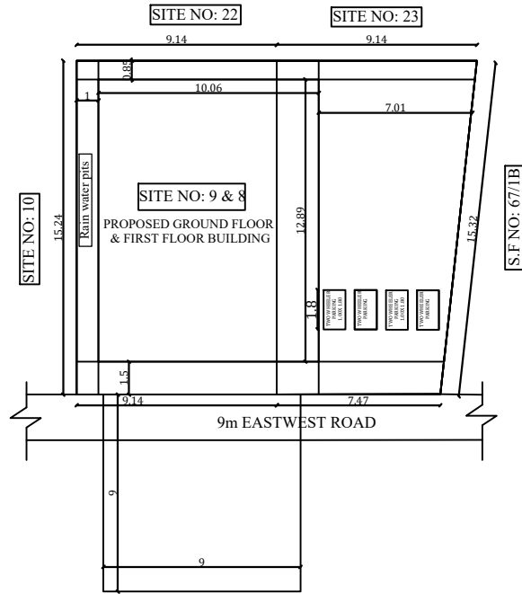
SITE PLAN
