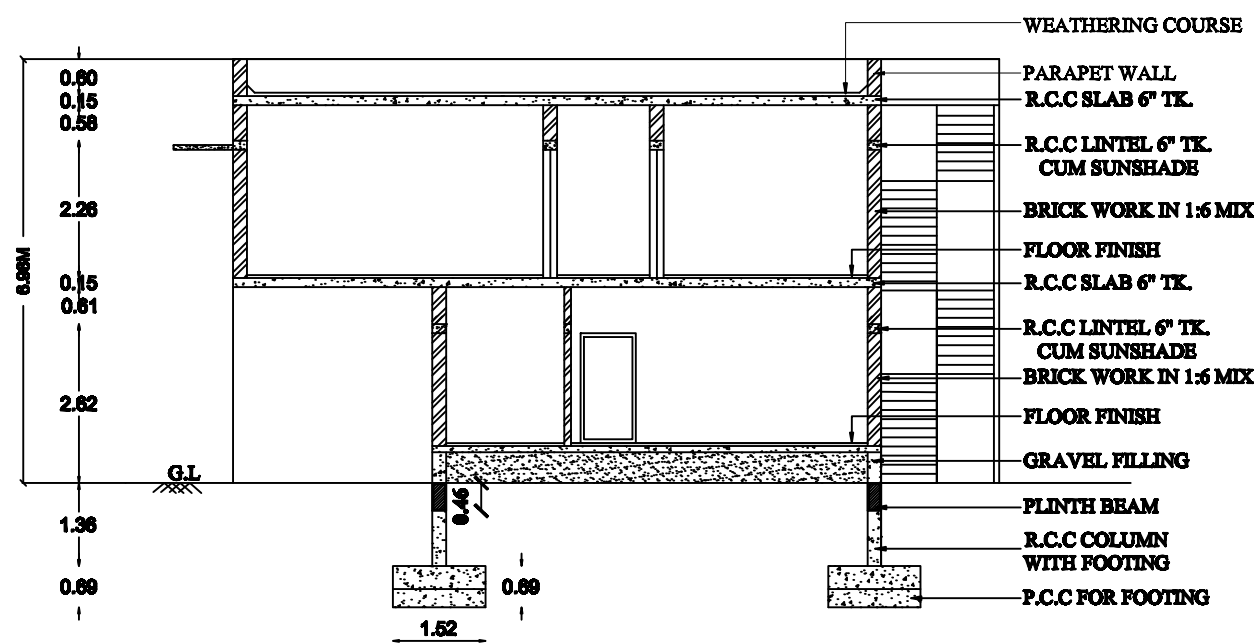
CROSS SECTION AT A-A
