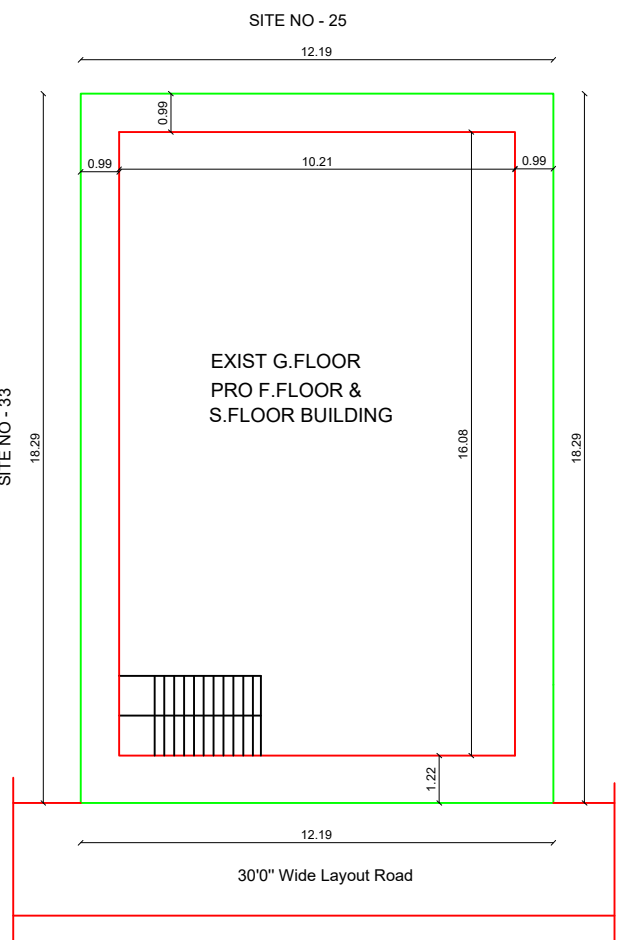
SITE PLAN
