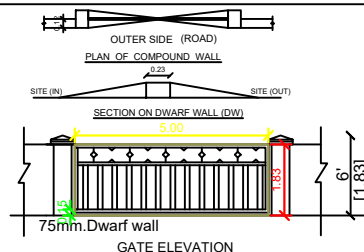
GATE ELEVATION
