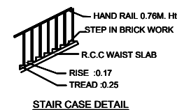
STAIR CASE DETAIL
