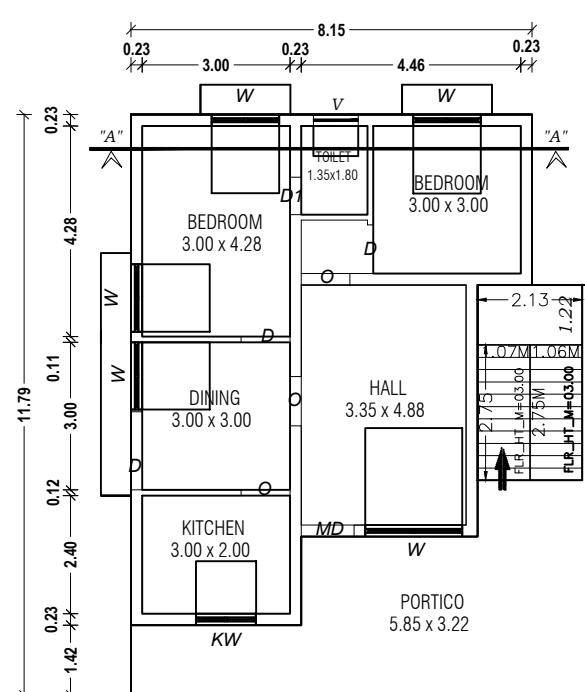
EX. GROUND FLOOR PLAN
