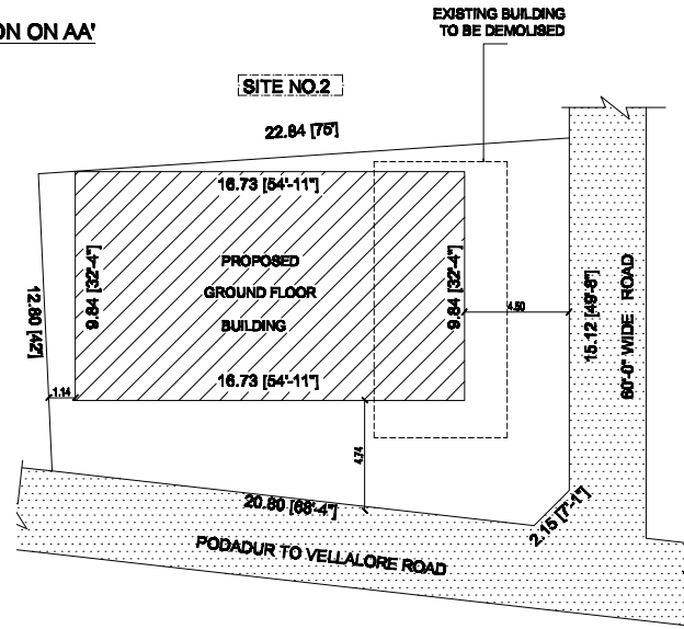
SITE PLAN
