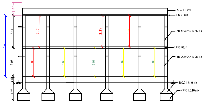
SECTION AB
