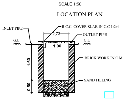
SECTIONAL DETAILS
