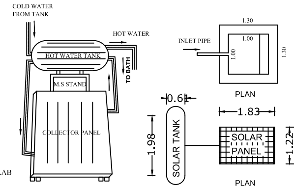
SOLAR WATER HEATER SYSTEM
