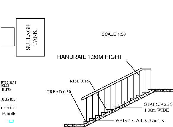
STAIRCASE DETAILS
