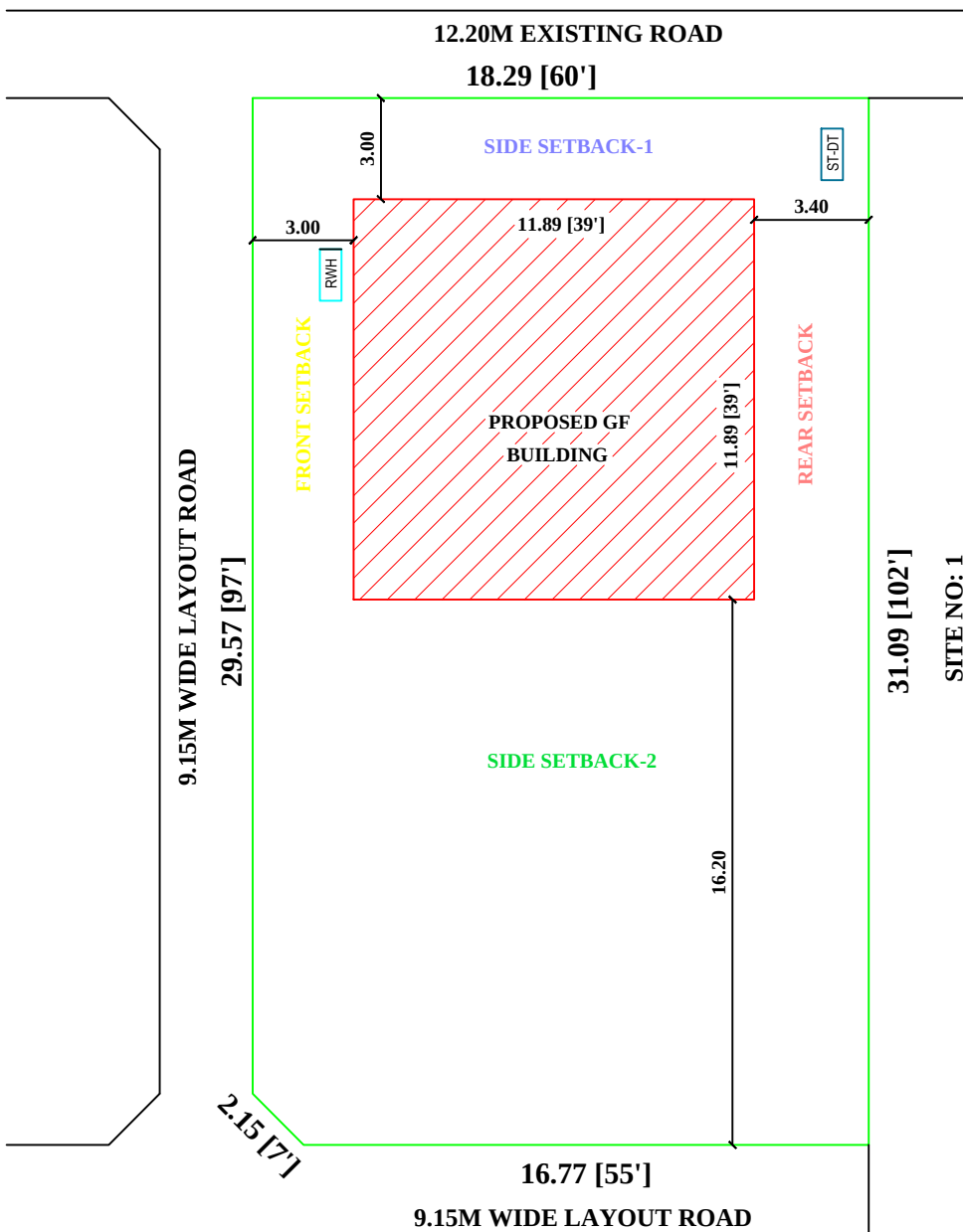
SITE PLAN
