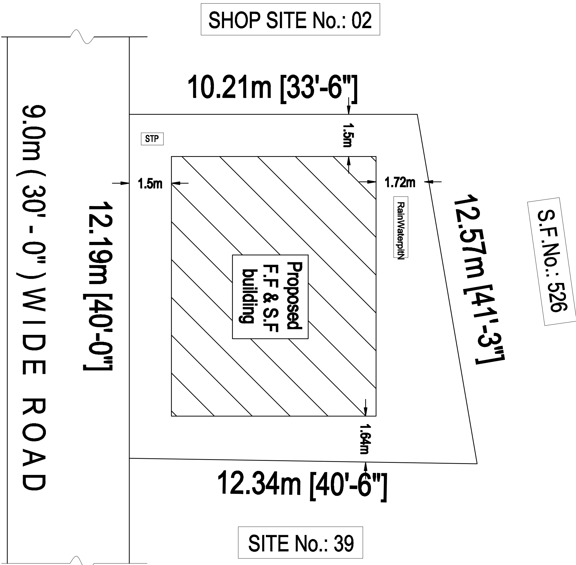
SITE PLAN
