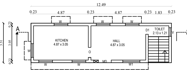
PROPOSED GROUND FLOOR PLAN
