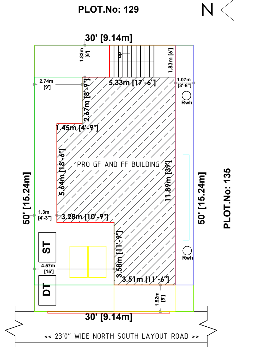
SITE PLAN
