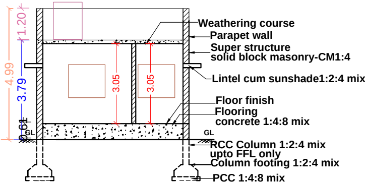
SECTION ELEVATION
