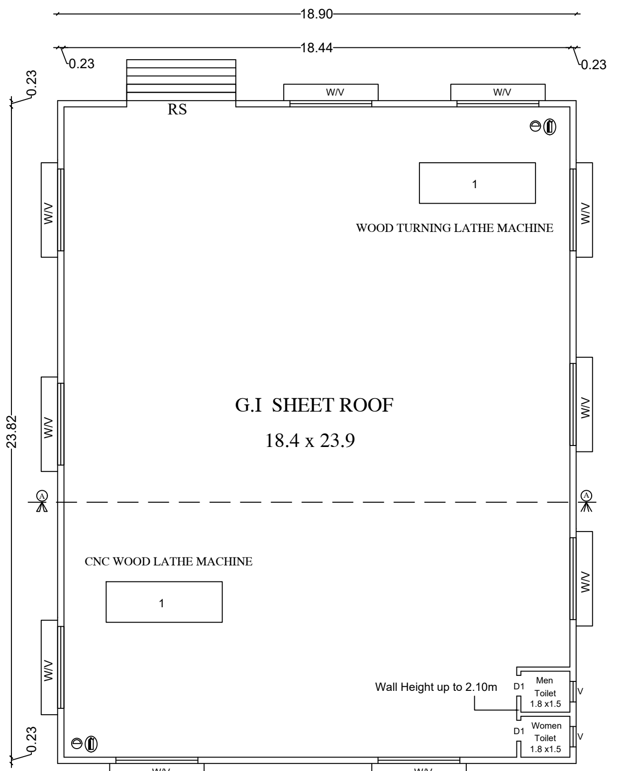
GROUND FLOOR PLAN (PROPOSED)
