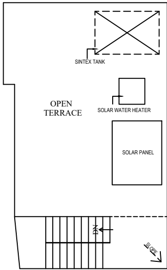
TERACE FLOOR PLAN
