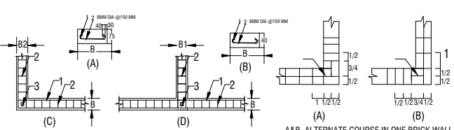
FIGURE 2: REINFORCEMENT AND BENDING DETAILS OF SEISMIC BANDS
