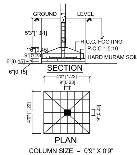
FOUNDATION DETAILS
