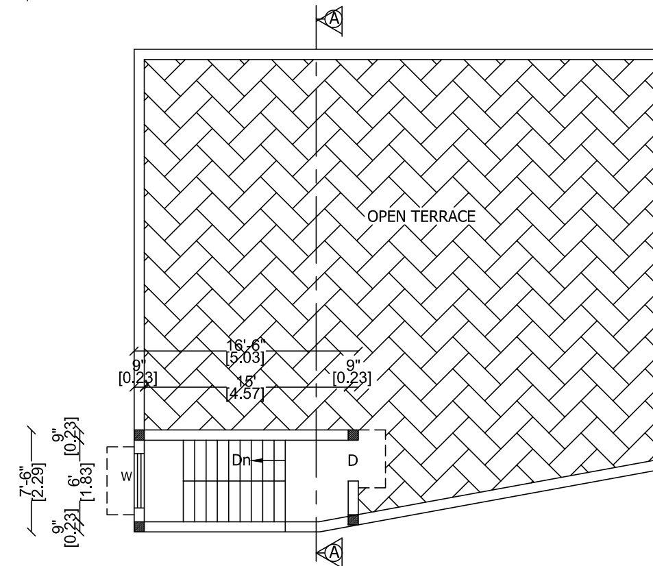
HEADROOM FLOOR PLAN
