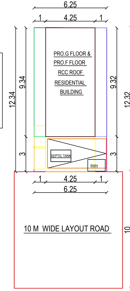
SITE PLAN
