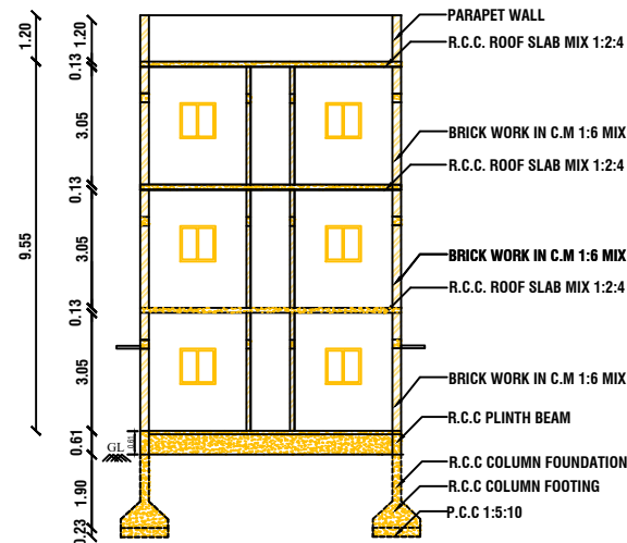
CROSS SECTION AT A-A
