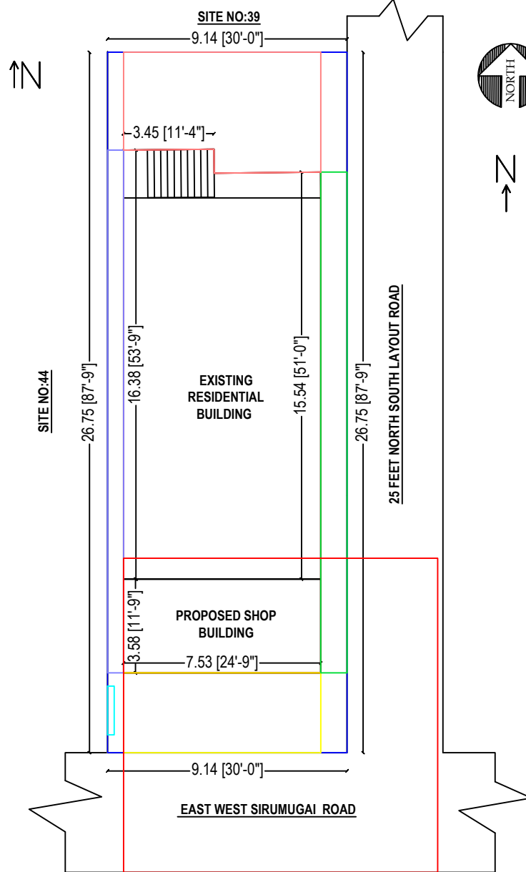
SITE PLAN
