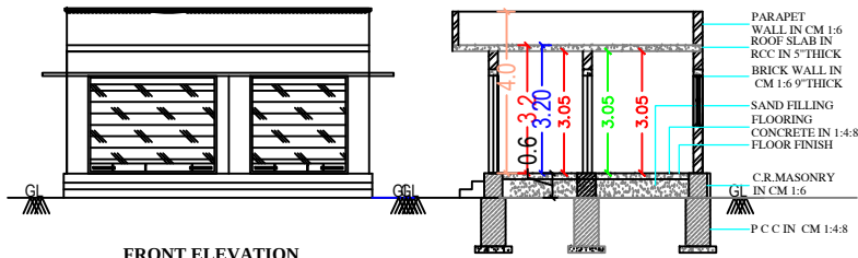
FRONT ELEVATION
