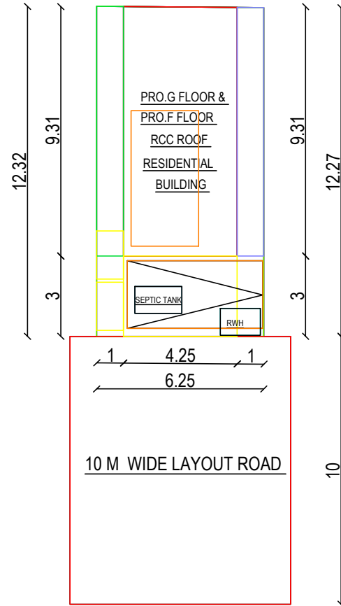
SITE PLAN
