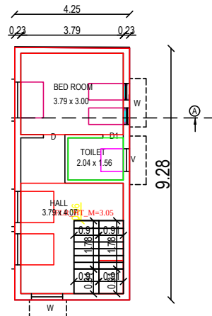
POSED FIRST FLOOR PLAN
