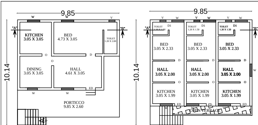
EXG & ADD. GROUND FLOOR
