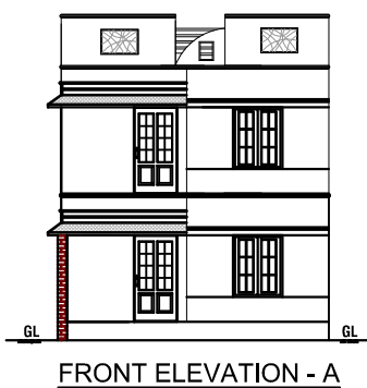
FRONT ELEVATION - A
