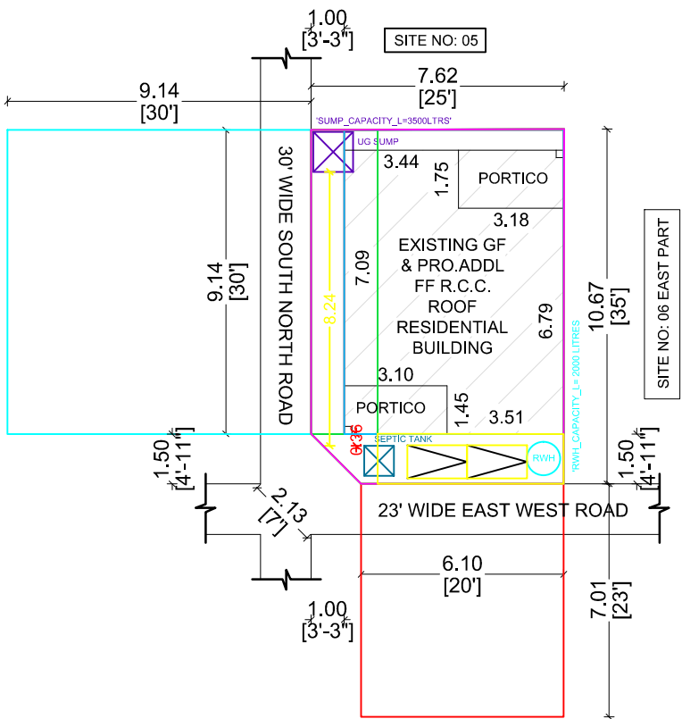
SITE PLAN
