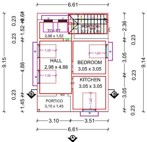
PROPOSED ADDITIONAL FIRST FLOOR PLAN
