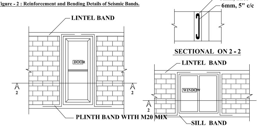
SECTIONAL ON 2-2 SCALE 1:50
