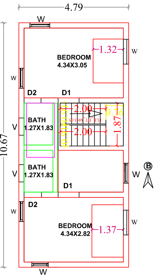
PRO. FIRST FLOOR
