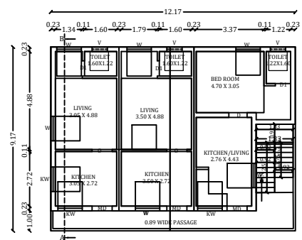
PRO.ADDL.FIRST FLOOR PLAN
