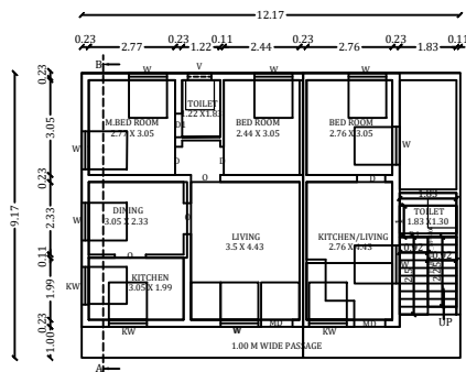
PRO.ADDL.GROUND FLOOR PLAN
