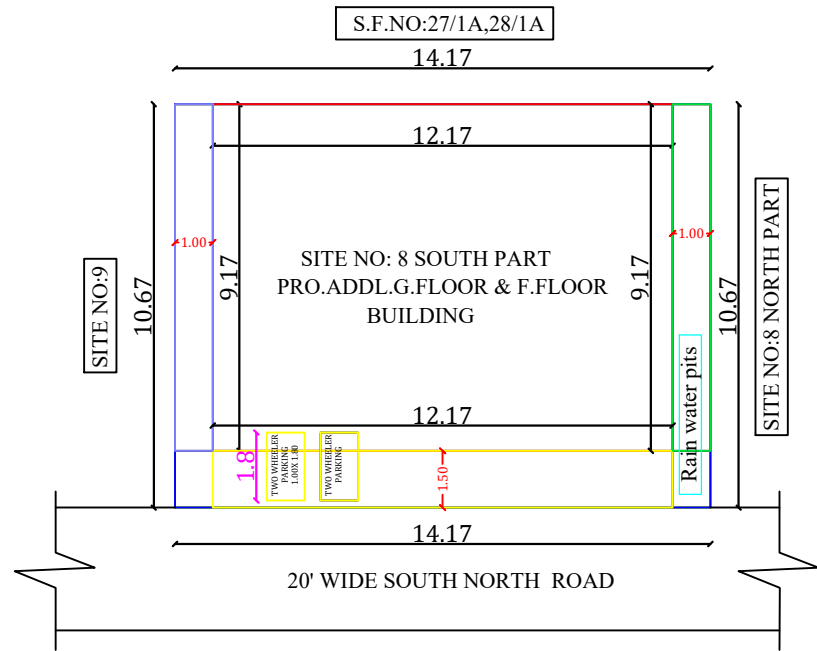
SITE PLAN
