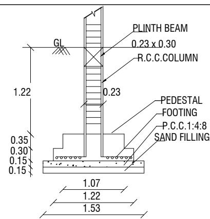
FOUNDATION DETAIL
