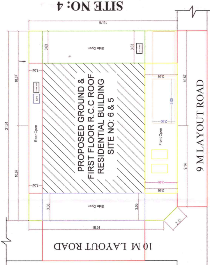
SITE PLAN
