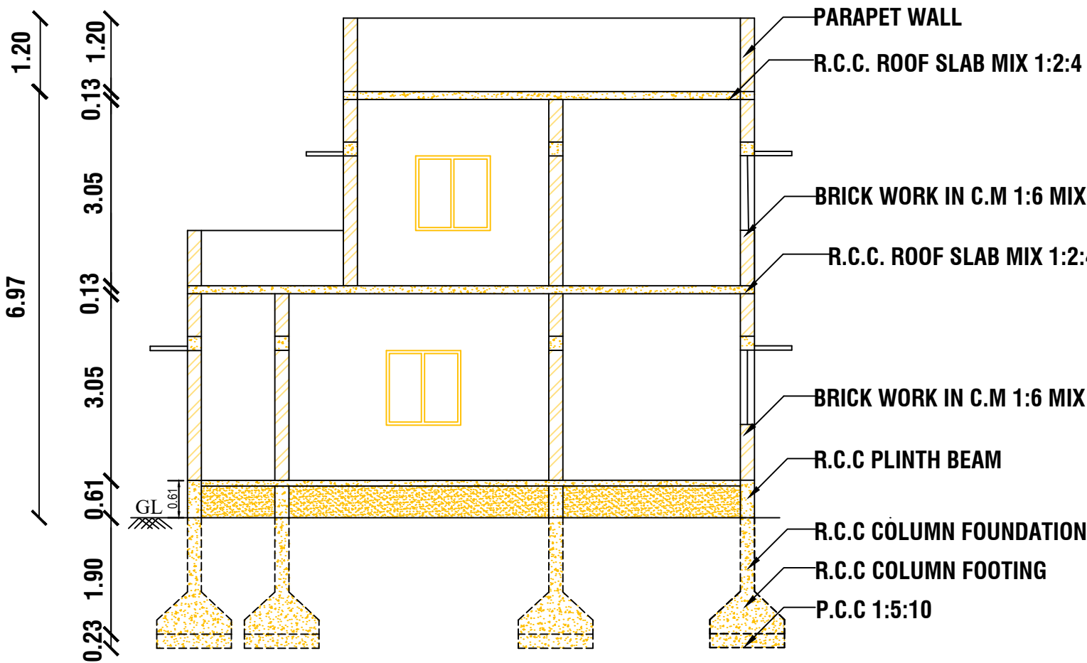
CROSS SECTION AT A-A
