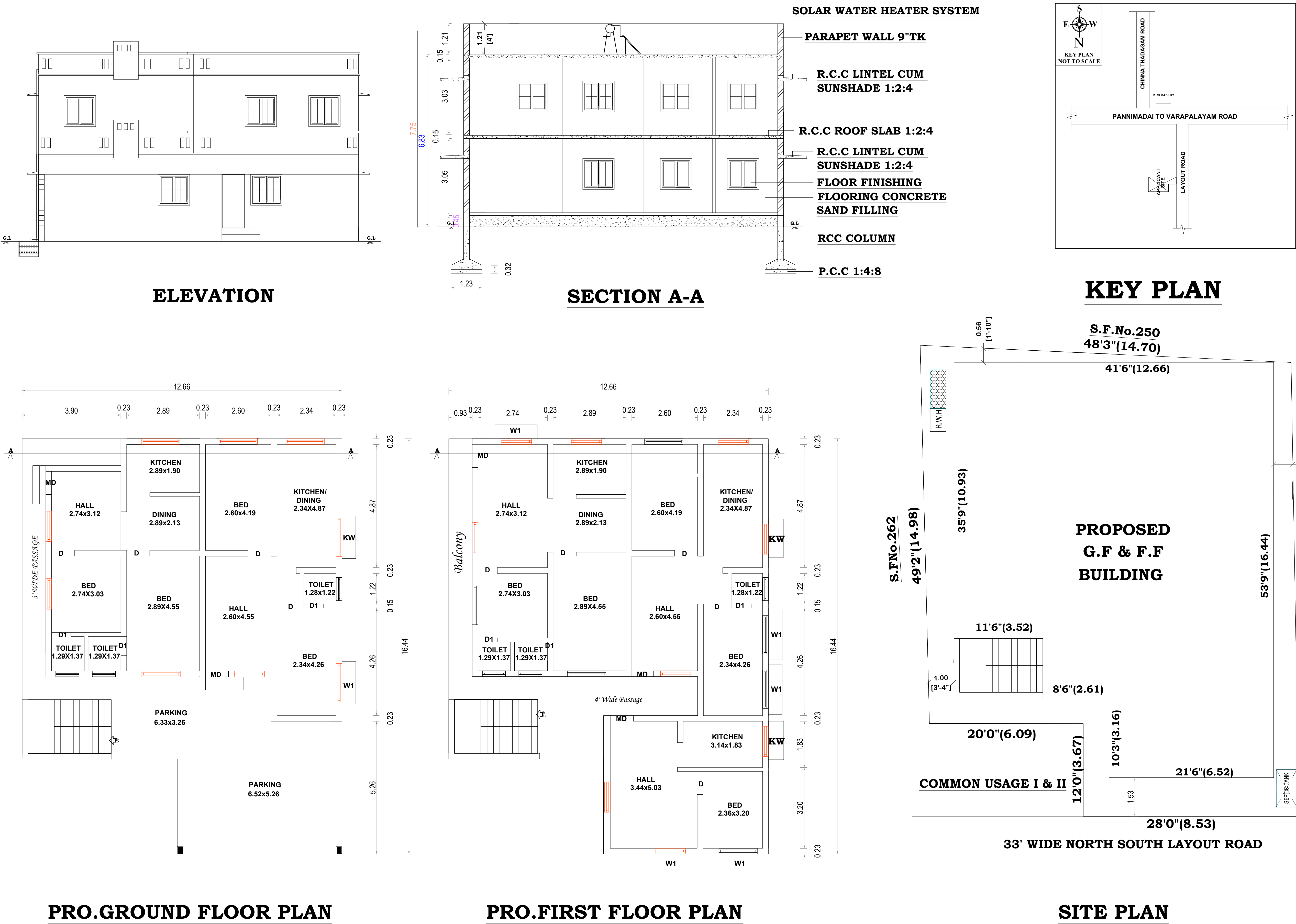
PRO.GROUND FLOOR PLAN
