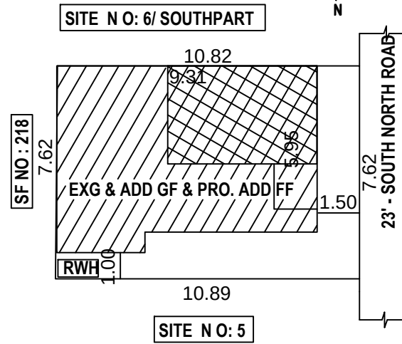
EXG & ADD. GROUND FLOOR
