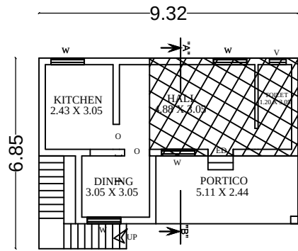
EXG & ADD. GROUND FLOOR
