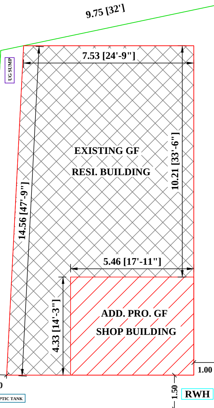
SITE PLAN
