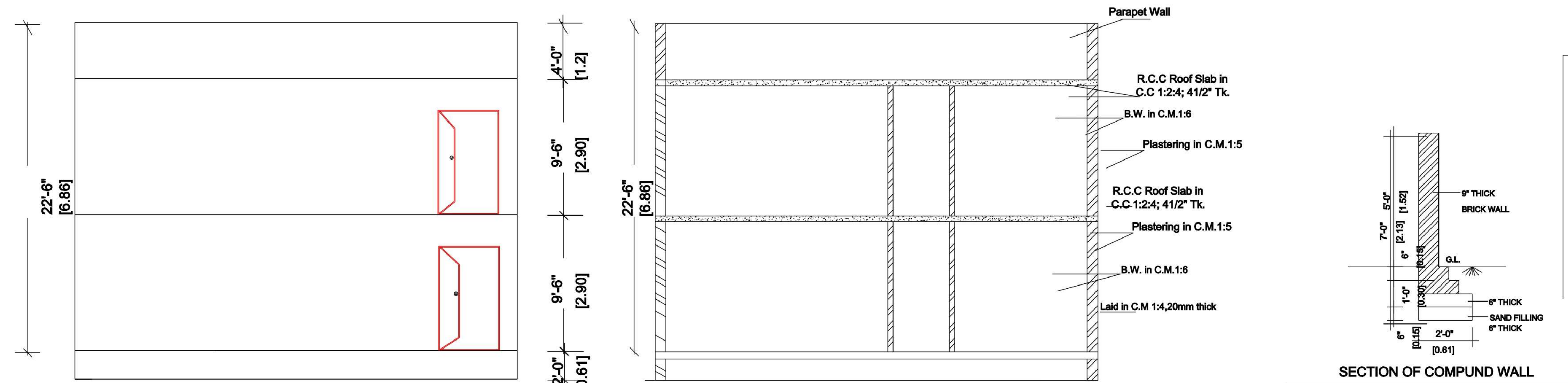
SECTION
