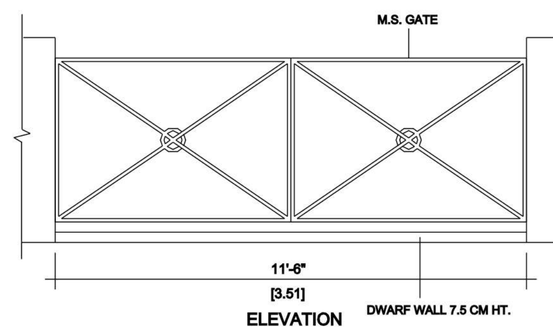
SCALE = 1 : 50
