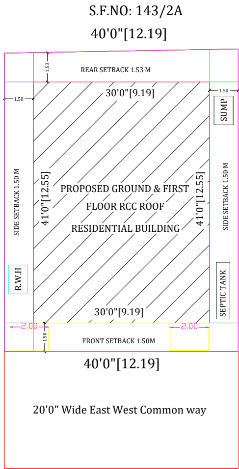
SITE PLAN
