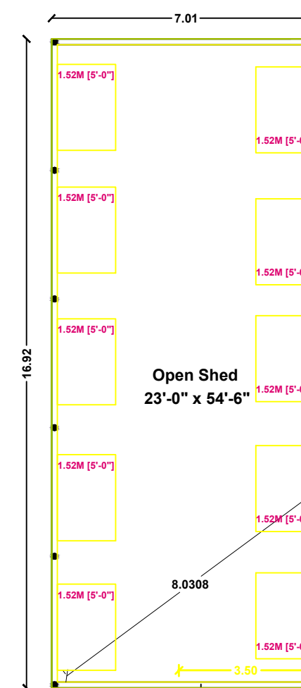
Shed Plan
