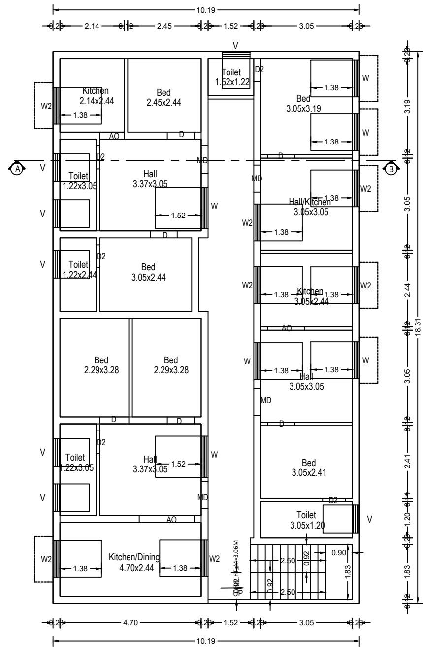
Plan Scale 1:100 Pro. First floor
